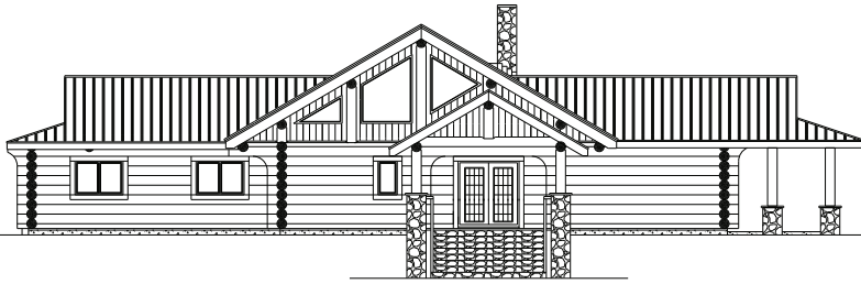
front elevation
