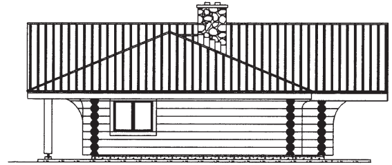
left elevation
